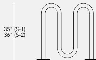
BIKE RACK 130 2-3/8" O.D. Tubing
