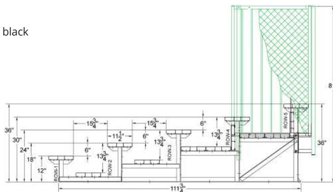
5-Row Deluxe Bleachers
