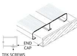
MODEL #AECIP-10 & AECIP12 End Cap with Tek Screws
