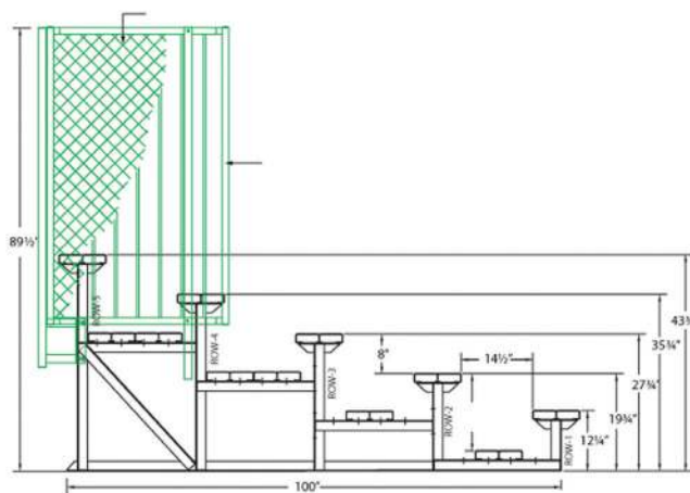
STANDARD 5-ROW BLEACHER DIMENSIONS
